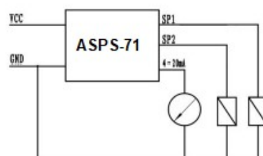
PNP output wiring diagram
