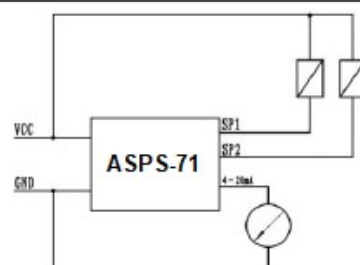
NPN output wiring diagram
